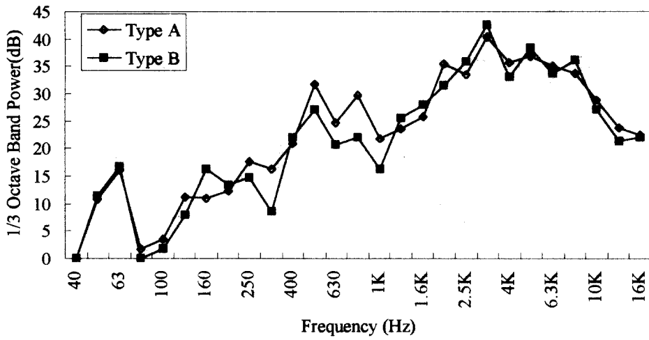
Fig. 10 Noise Spectrum in ASHRAE Condition
