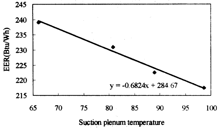
Fig. 4 Suction Plenum Temperature vs EER
