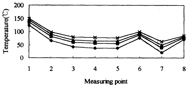
Fig. 3 Temperature Distribution of Measure Points (■ : Normal Condition)
