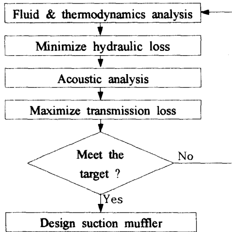
Fig. 1 Diagram of Muffler Design
