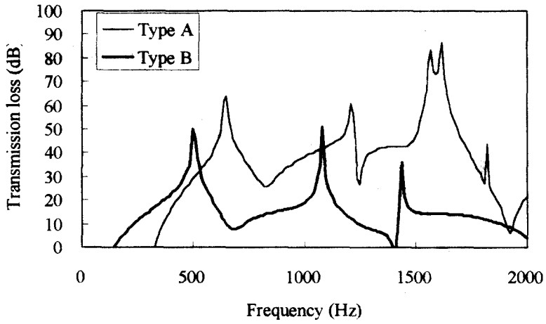
Fig. 8 Calculated Result of Muffler Transmission Loss
