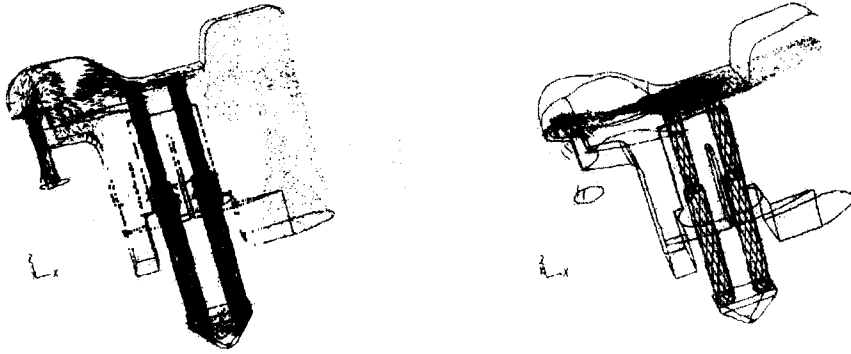
Fig. 7 Flow Field of Type B Muffler
