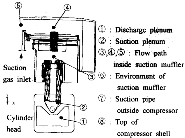
Fig. 2 Temperature Measuring Point in Suction Muffler
