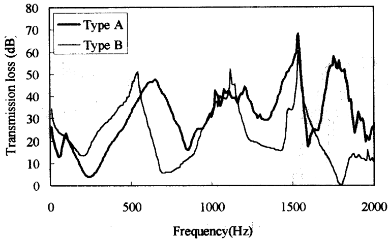
Fig. 9 Experimental Result of Muffler Transmission Loss
