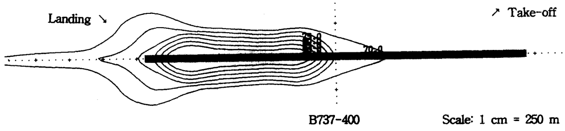
Figure 2. WECPNL Contour for Aircraft Types.
