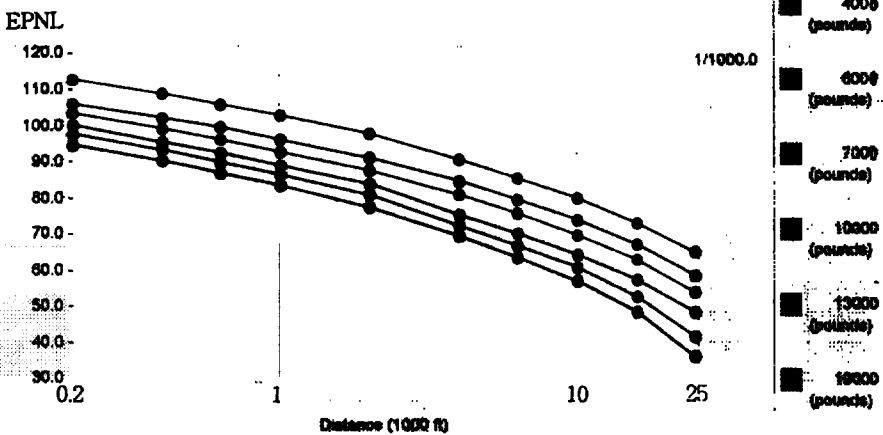
Figure 1. Effective perceived noise level for distance according to engine thrust.
