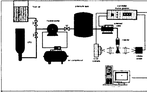
Fig. 1 Experimental setup
