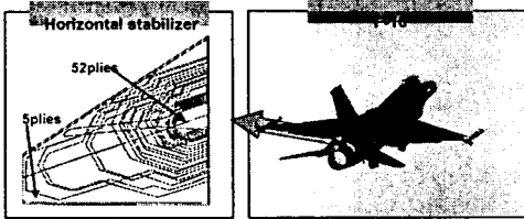
Fig. 1 Plydrops in the horizontal stabilizer of General Dynamics F-16 A/B.
