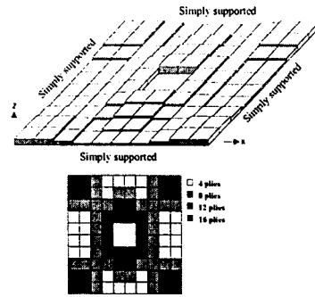
Fig. 6 Thickness distribution and contour of composite plate.
