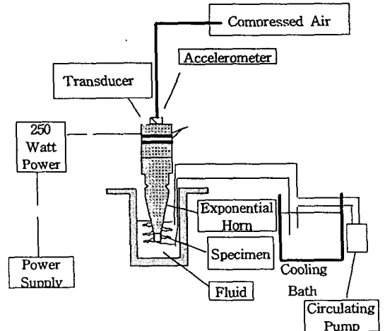
Fig. 2 Schematic diagram of cavitation-erosion test apparatus
