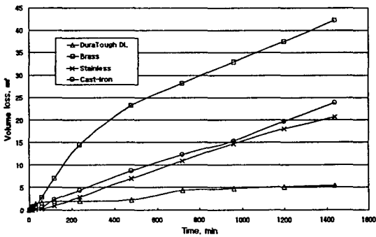
Fig.4 Volume loss vs testing time in distilled-water
