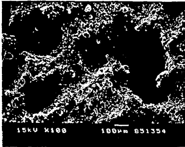
(b) Brass, × 100
