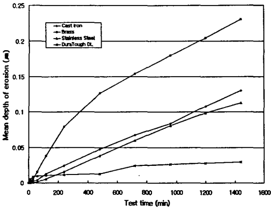
Fig.3 Mean depth of erosion as a function of cavitation erosion test time
