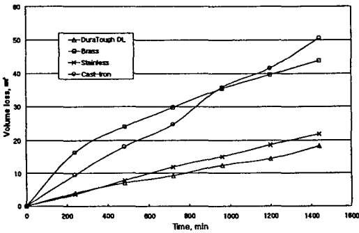
Fig.5 Volume loss vs testing time in sea-water
