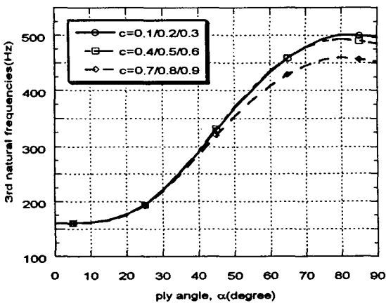
Fig. 5 Variation of the natural frequencies with ply angle for congregated cracks at different positions ( \bar{a}_i=0.2 , \nu_f=0.5 )
