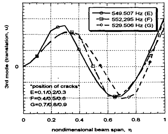
Fig. 6 First three mode shapes for congregated cracks at different positions ( \bar{a}_i=0.2 , \nu_f=0.5 , \alpha=90^\circ )
