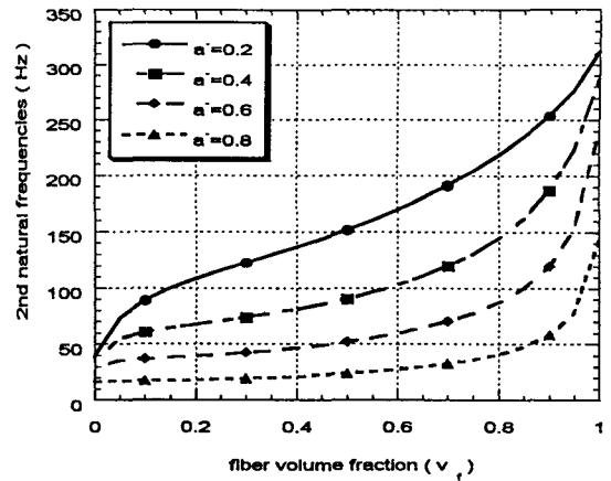
Fig. 8 Variation of the 2nd natural frequencies with fiber volume fraction for different crack depths ( n=5(D) , \alpha=90^\circ )
