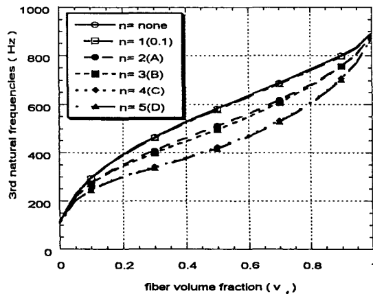
Fig. 7 Variation of the natural frequencies with fiber volume fraction for different crack numbers and positions ( \bar{a}_i=0.2 , \alpha=90^\circ )
