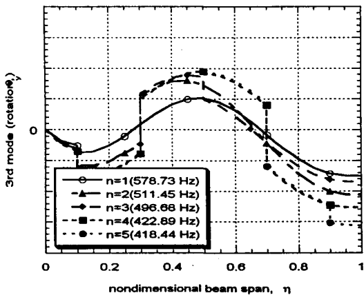
Fig. 9 Rotational mode shapes for the different crack numbers and positions
