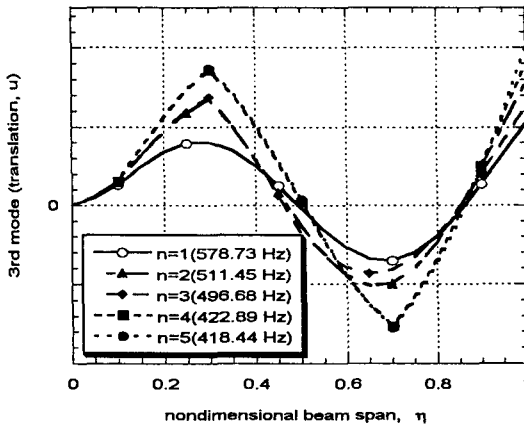
Fig. 3 First three mode shapes for different crack numbers and positions ( \bar{a}_i=0.2 , c_i=0.1, 0.3, 0.5, 0.7, 0.9 , \nu_f=0.5 )
