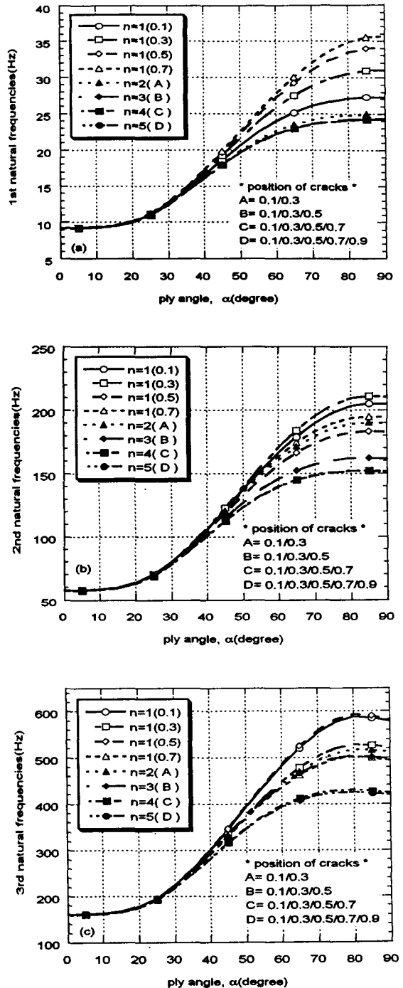
Fig. 2 Variation of the natural frequencies with ply angle for different crack numbers and positions ( \bar{a}_f=0.2 , c_f=0.1, 0.3, 0.5, 0.7, 0.9 , \nu_f=0.5 )
