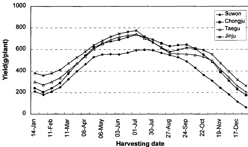
Fig. 1. Yield per plant for each harvest date.
