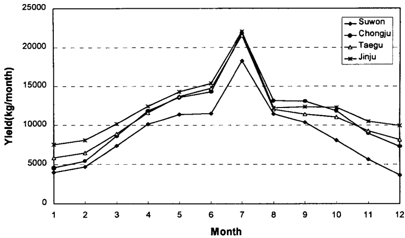
Fig. 2. Total yield per month.
