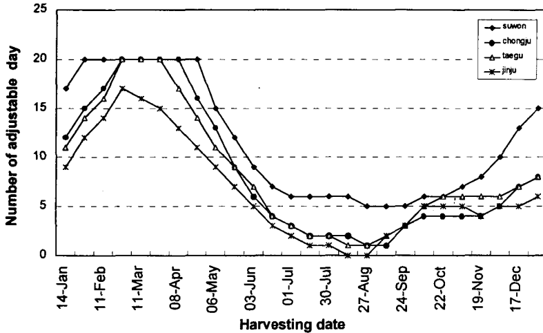
Fig. 3. Number of maximum adjustable days for yielding date.
