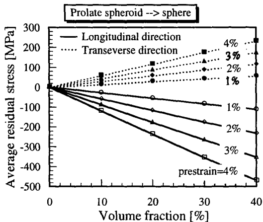
Fig.5 Average residual stresses of Al matrix as a function of volume fraction of TiNi particle. Composite is given a tensile strain in longitudinal direction.
