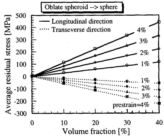
Fig.6 Average residual stresses of Al matrix as a function of volume fraction of TiNi particle. Composite is given a compressive strain in longitudinal direction.
