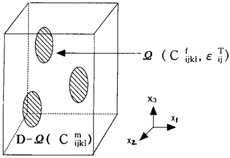
Fig.4 Analytical model for calculating average residual stress in the matrix.
