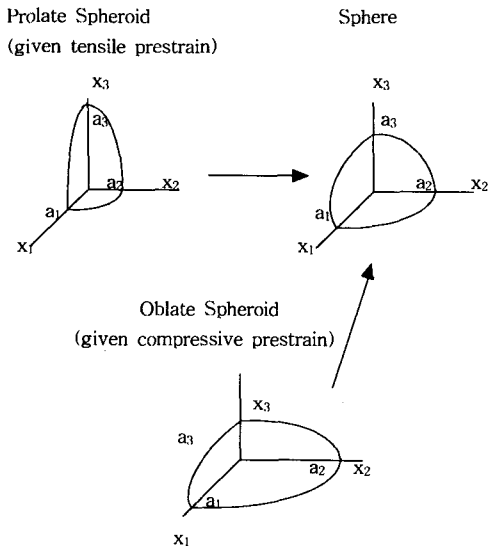
Fig.3 Calculation of strain by the shape memory effect.
