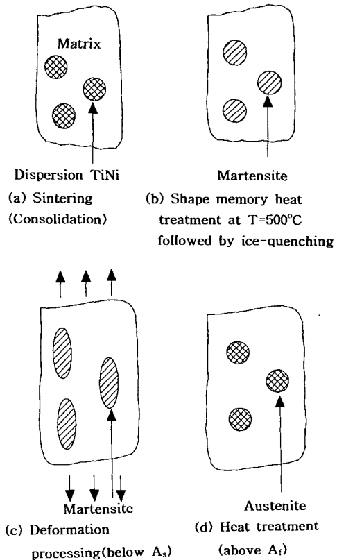
Fig.2 Strengthening mechanism of composite by the shape memory effect
