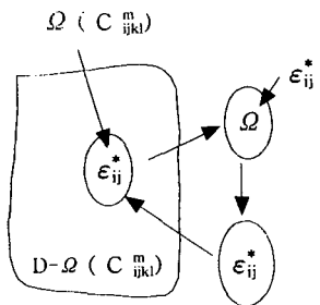
Fig.1 Eshelby's solution
