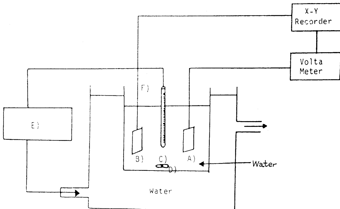
Fig.2. Experimental apparatus.
