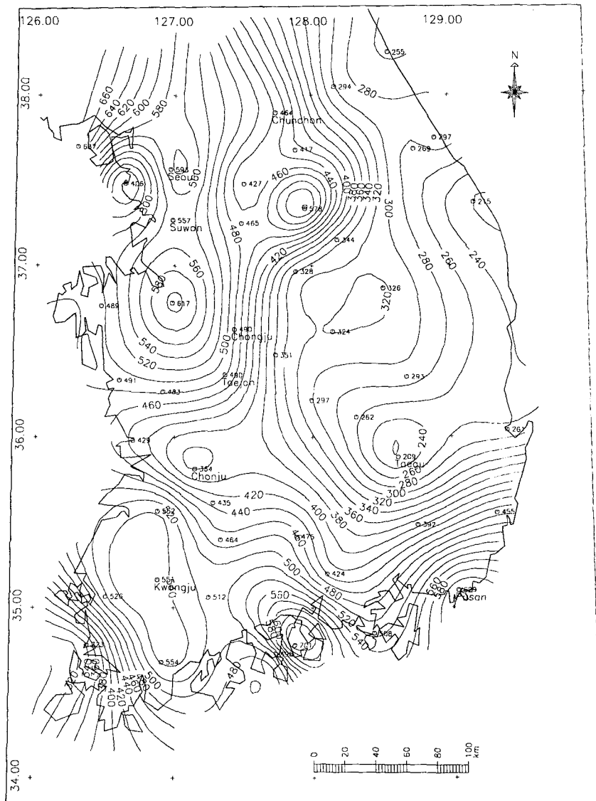
Annual R in Korea
