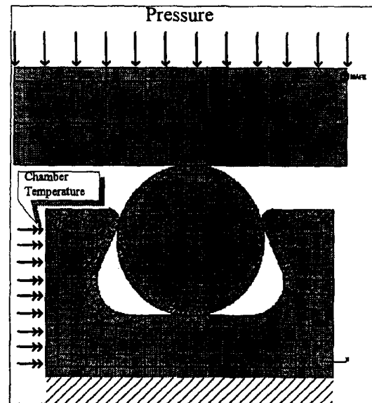
Fig. 1 Mesh generation and boundary conditions of an O-ring seal
