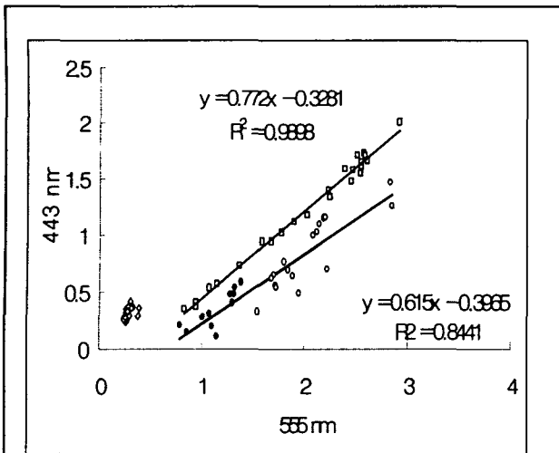
Fig. 9 Scattered plot of the four spectra types on 443-555nm plane. diamonds: open water, rectangles: high SS water, filled circles: red tide water with less SS, and open circles: red tide water with high SS.
