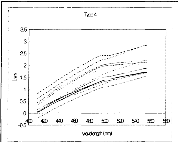
Fig. 8. L_{WN} spectra of red tide pixels with high level with SS.
