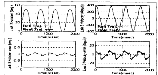
Fig. 10. The experimental results of SOFC for position and velocity trajectory tracking of link 3 with no payload.
