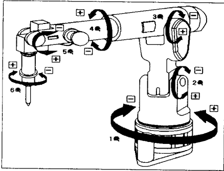
Fig. 3. Coordinates frame of AC1 robot.
