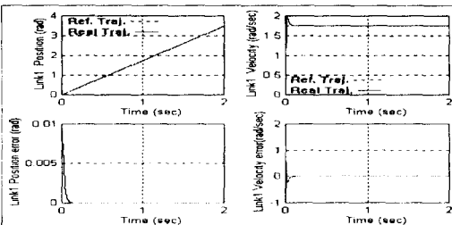
Fig. 8. Simulation results of position and velocity trajectory tracking for link 1 with 4kg payload in case of ramp input.
