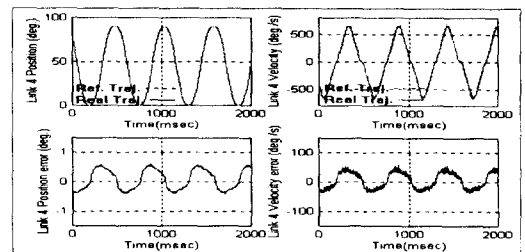
Fig. 11. The experimental results of SOFC for position and velocity trajectory tracking of link 4 with no load.
