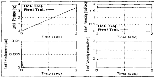
Fig. 6. Simulation results of position and velocity trajectory tracking for link 1 with no load in case of ramp input.
