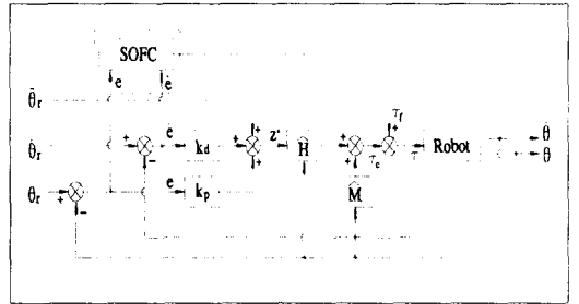
Fig. 2. The block diagram of proposed self-organizing fuzzy control structure for robot manipulator.
