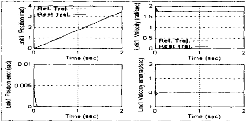
Fig. 7. Simulation results of position and velocity trajectory tracking for link 1 with 2kg payload in case of ramp input.
