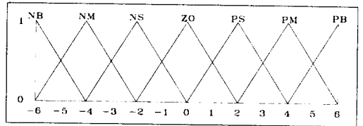
Fig. 4. Linguistic variable.
