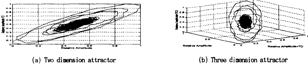
Fig. 11 Attractor reconstruction for part of web signal(side hole)
