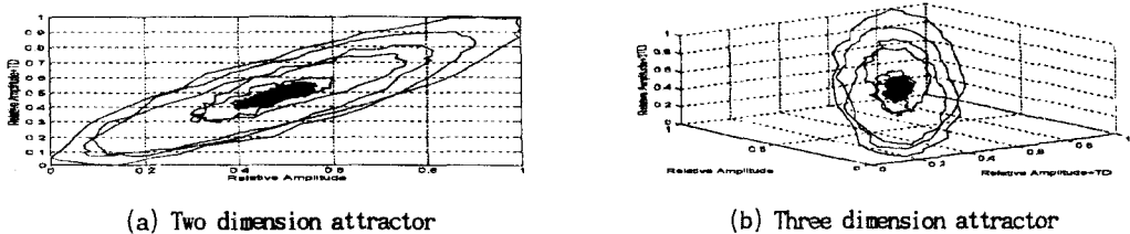
Fig. 12 Attractor reconstruction for part of flange signal(crack)
