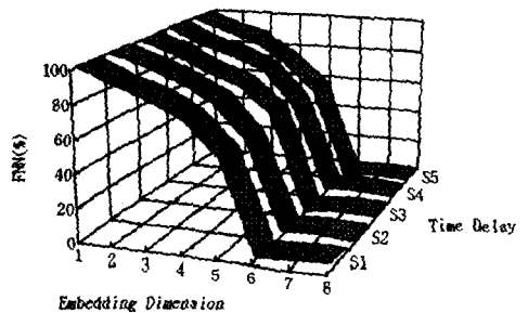
Fig. 9 Determination of embedding dimension
