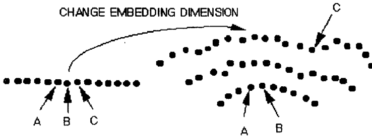
Fig. 1 Concept of false nearest neighbor
