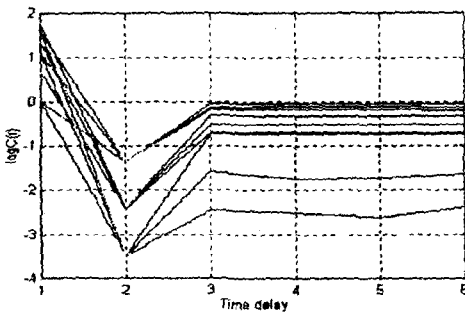
Fig. 8 Determination of time delay
