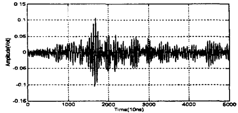
Fig. 5 Defect signal for head part (slit type crack)
