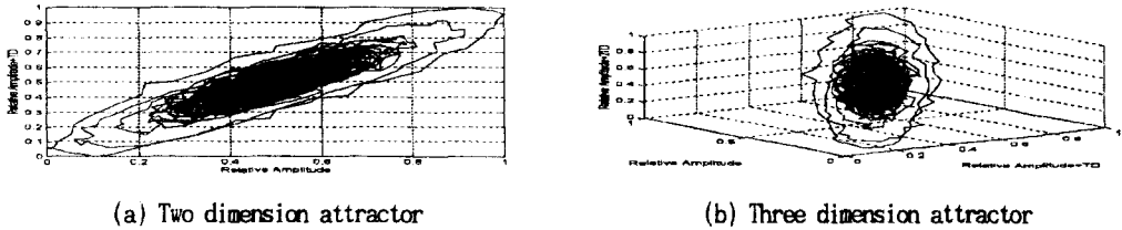
Fig. 10 Attractor reconstruction for part of head signal(crack)
