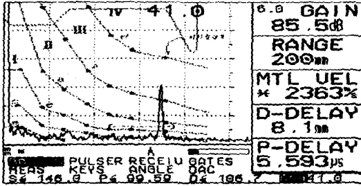
(a) defect signal on ultrasonic equipments
