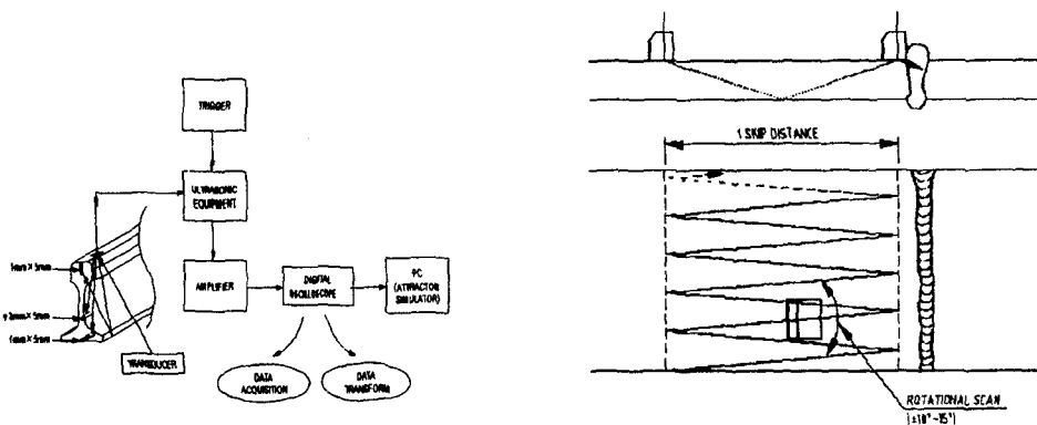
Fig. 2 Schematic of data acquisition and Fig. 3 Schematic of ultrasonic scan for defect detection
