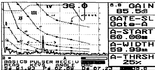
(a) defect signal on ultrasonic equipments
