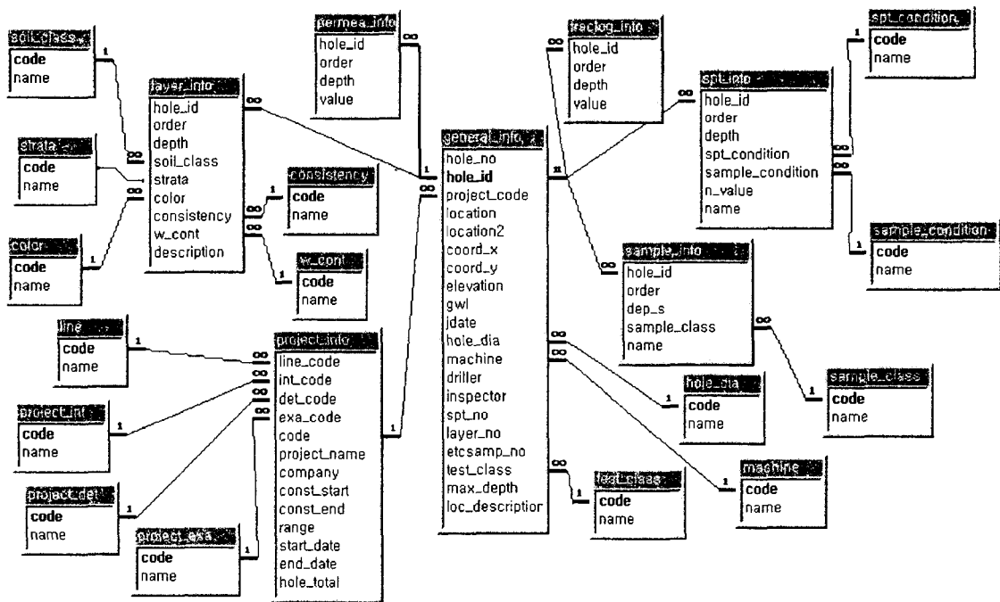
Fig. 2 Relational Structure of HGIS Database
