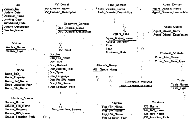
<Figure 1> Repository Schema for HyDoMIS
