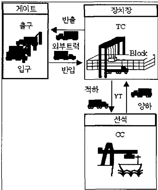
Fig 2.1 Container Terminal System
