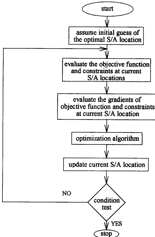
Fig. 2 Flow Chart for Optimization of S/A Placement
