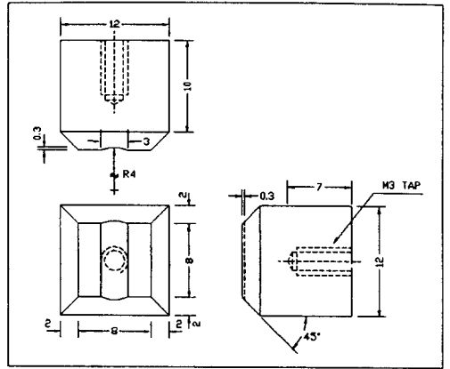
Fig. 3 Schematic diagram of plant contacting part
