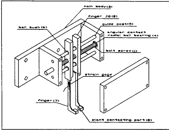
Fig. 2 Schematic diagram of a soft gripper
