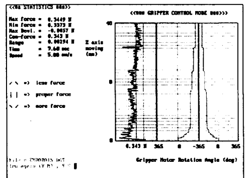
Fig. 8 The result of gripping control during the extraction
