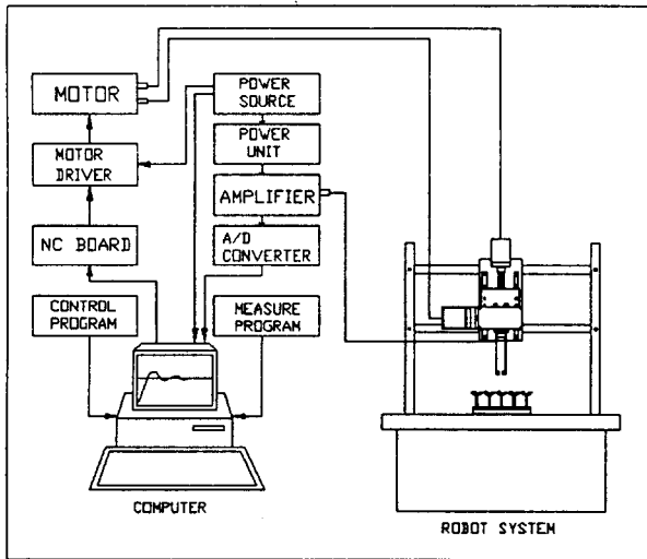
Fig. 4 Schematic diagram of control system of gripper
