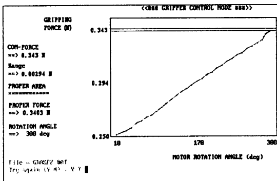
Fig. 7 The result of gripping control during the gripping
