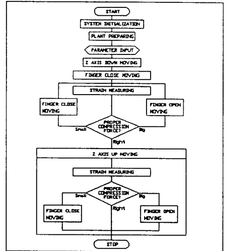
Fig. 5 The flow-chart of control program of soft gripper
