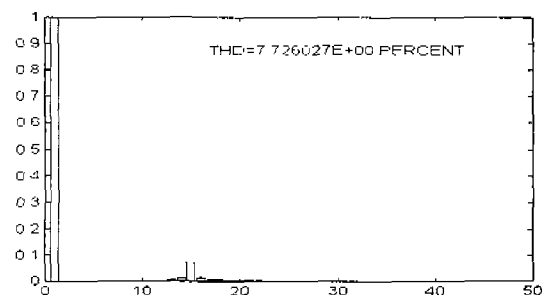
Fig. 12: Harmonic Spectrum of the Input Phase Current in the 3-wired Hui's Flyback Converter
