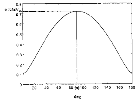
Fig. 4 V_{m,rms} at phase delay angle \alpha
