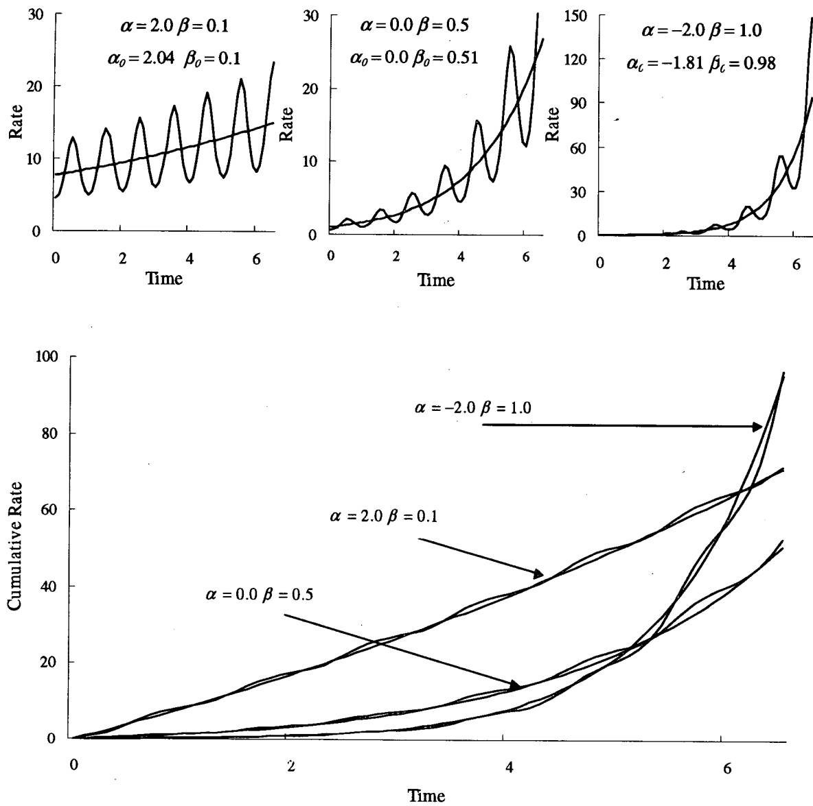
Figure 3. Estimated EPF rate functions for system failure processes with cyclic behavior corresponding to EPTF-type rate function of A = 0.5 and \omega = 1.0 .
