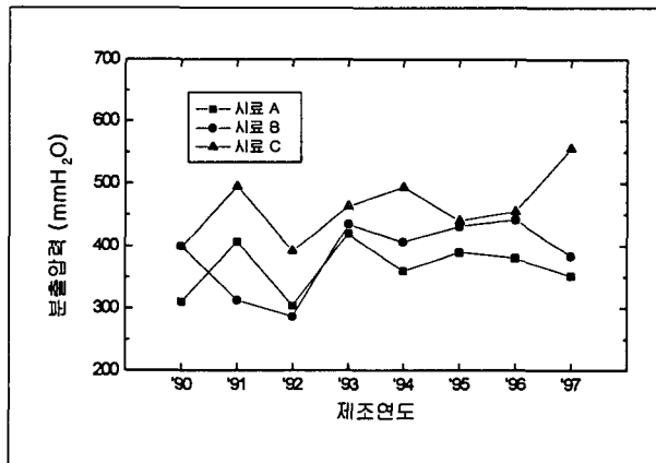
Fig. 3 Popping pressure distributions of safety valves as a function of a manufacture year
