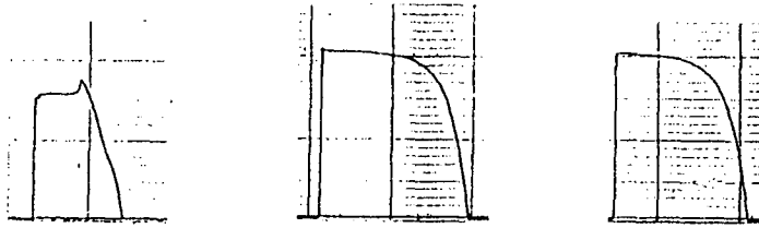
(a) 시료 A (b) 시료 B (c) 시료 C Fig. 4 Measurement of popping modes in safety valves
