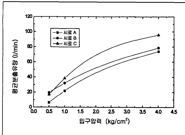
Fig. 6 Average flow rate of the safety valve
