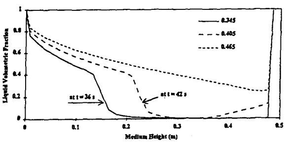
Fig. 3 Effect of porosity on the axial saturation distribution: P_{sys} = 1 atm, H = 0.485 m, d_p = 3 mm and q''' = 3 MW/m 3 with uniform heat profile.
