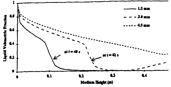
Fig. 5 Effect of particle size on the axial saturation distribution: P_{sys} = 1 atm, H = 0.485 m, \epsilon = 0.405 and q''' = 3 MW/m 3 with uniform heat profile.
