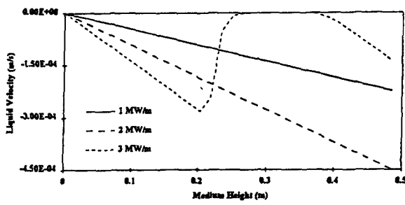
Fig. 2 Effect of heat generation rate on the axial liquid superficial velocity distribution at t = 43.5 s: P_{sys} = 1 atm, H = 0.485 m, d_p = 3 mm and \epsilon = 0.405 with uniform heat profile.
