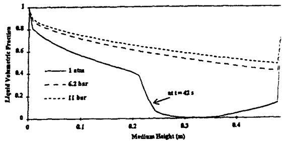
Fig. 7 Effect of system pressure on the axial saturation distribution: H = 0.485 m, d_p = 3 mm, \epsilon = 0.405 and q''' = 3 MW/m 3 with uniform heat profile.
