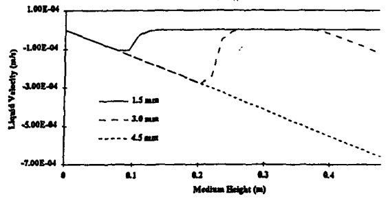
Fig. 6 Effect of particle size on the axial liquid superficial velocity distribution: P_{sys} = 1 atm, H = 0.485 m, \epsilon = 0.405 and q''' = 3 MW/m 3 with uniform heat profile.
