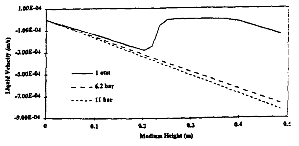
Fig. 8 Effect of system pressure on the axial liquid superficial velocity distribution: H = 0.485 m, d_p = 3 mm, \epsilon = 0.405 and q''' = 3 MW/m 3 with uniform heat profile.
