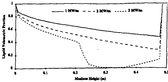
Fig. 1 Effect of heat generation rate on the axial saturation distribution at t = 43.5 s: P_{sys} = 1 atm, H = 0.485 m, d_p = 3 mm and \epsilon = 0.405 with uniform heat profile.
