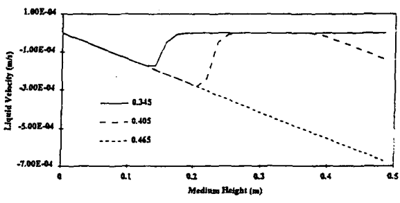
Fig. 4 Effect of porosity on the axial liquid superficial velocity distribution: P_{sys} = 1 atm, H = 0.485 m, d_p = 3 mm and q''' = 3 MW/m 3 with uniform heat profile.
