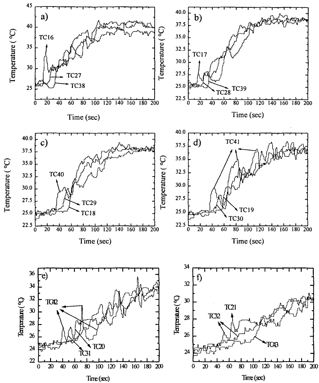
Fig.3 Temperature records at the same level
