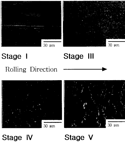
Fig. 8. SEM images of tested ball surfaces for each stage.
