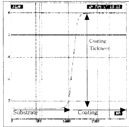
Fig. 4. An example of coating thickness measurement using Alpha-step.
