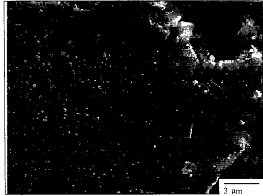
Fig. 10. SEM image of a tested ball surface for stage V.
