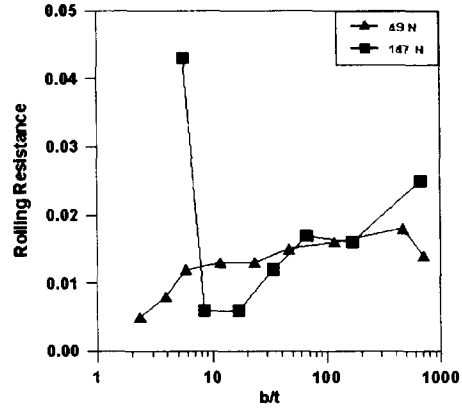
Fig. 6. Rolling resistance vs. b/t value after the failure of silver film (stage IV).
