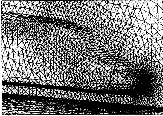
Fig. 4 Mesh configuration at train nose for steady state simulation(real case)
