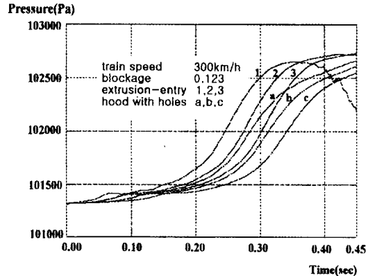
Fig. 7 Pressure time-history in tunnel for extrusion-entry & hood with holes
