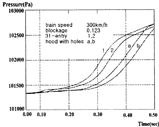
Fig. 8 Pressure time-history in tunnel for 31-entry & hood with holes
