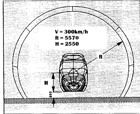
Fig. 2 Picture of cross-sectional area for train and tunnel
