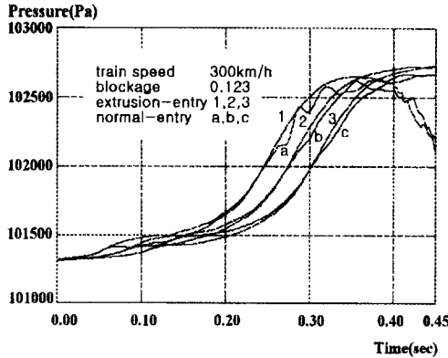
Fig. 6 Pressure time-history in tunnel for extrusion-entry & normal-entry
