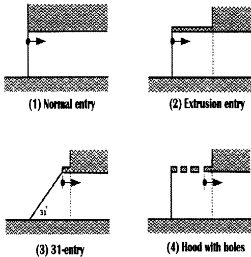
● numerical sensor is located from this point Fig. 3-1 Tunnel entry shapes calculated this study
