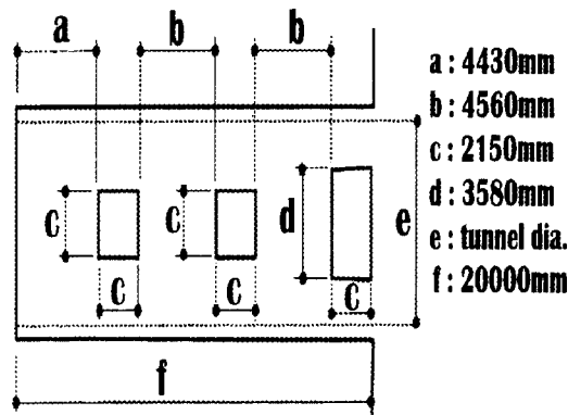
Fig. 3-2 Specifications of hood with holes
