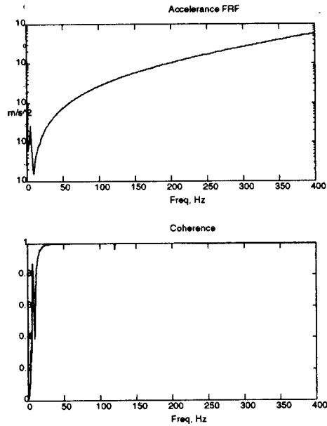
Fig. 5 FRF of acceleration and its coherence
