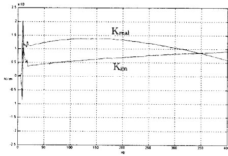
Fig.7 Real and imaginary part of dynamic stiffness
