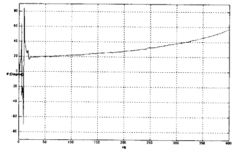
Fig.10 Phase, \theta between E_{real} and E_{im}
