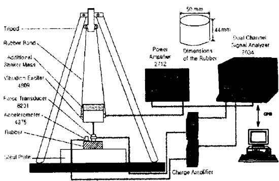
Fig. 4 Experimental test setup
