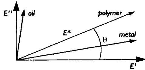
Fig. 2 Elastic modulus and loss modulus
