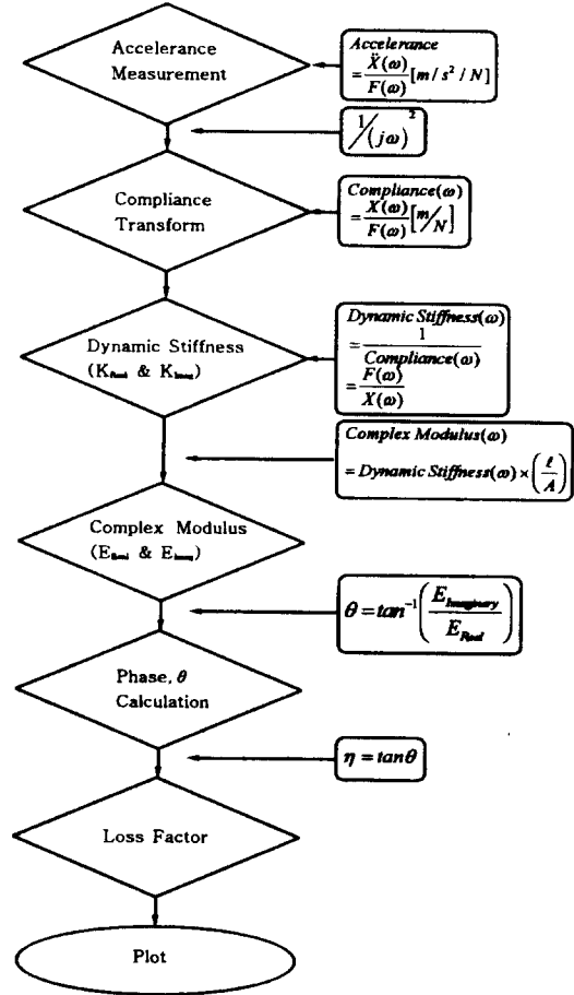
Fig. 3 Test flowchart for impedance method
