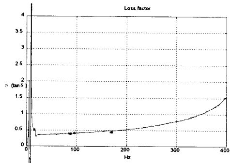
Fig.11 Loss factor
