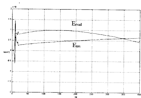
Fig.9 Real and imaginary part of complex modulus
