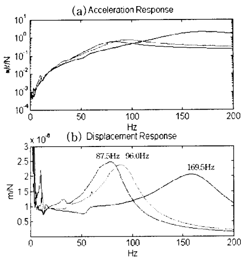
Fig. 12 FRF of acceleration and displacement
