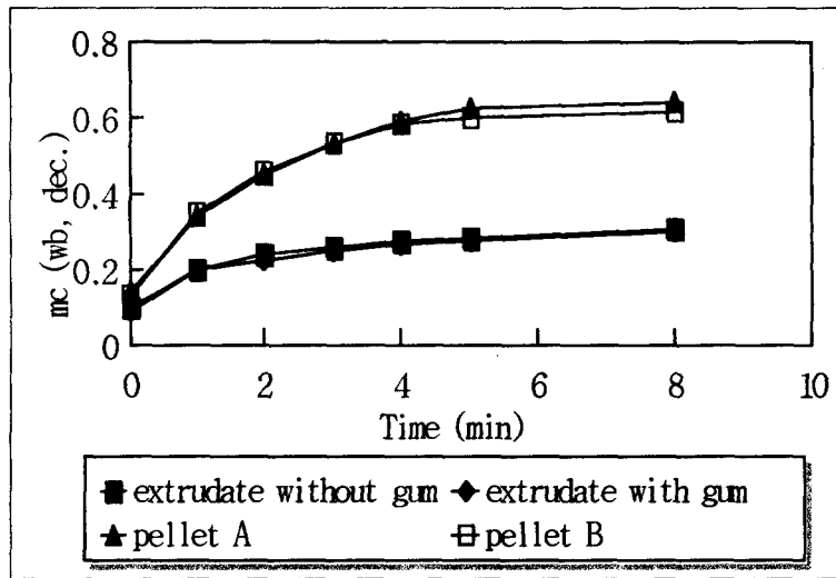
Fig. 2. Water holding capacity of different fish feeds after sinking.
