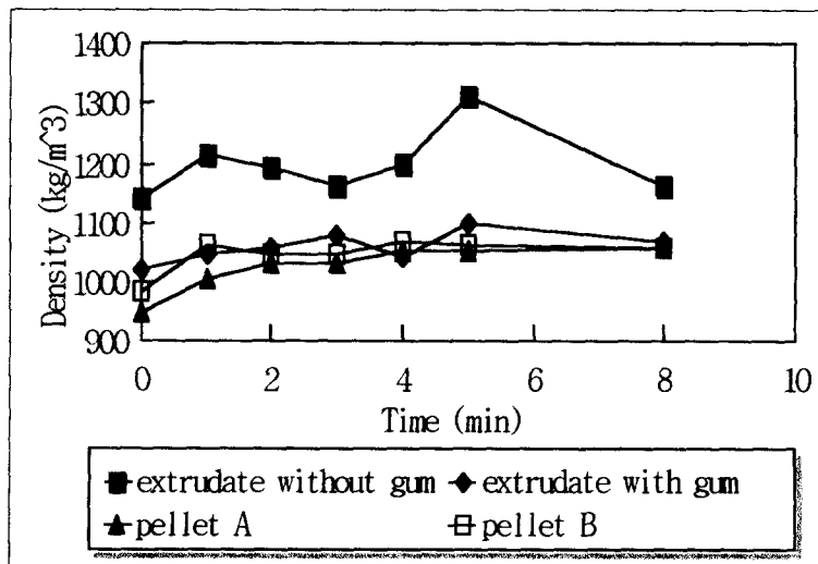
Fig. 4. Density of different fish feeds after sinking.
