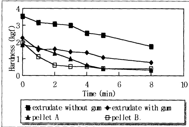
Fig. 3. Hardness of different fish feeds after sinking.
