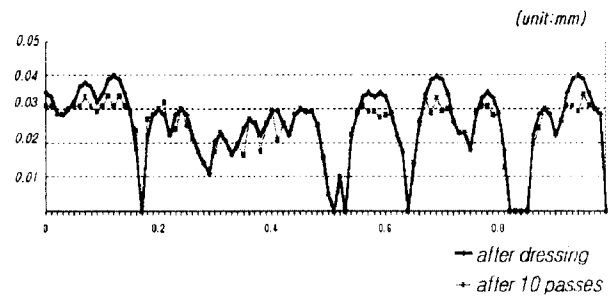
Fig. 7 Comparison of simulated profiles of after dressing and after 10 passes
