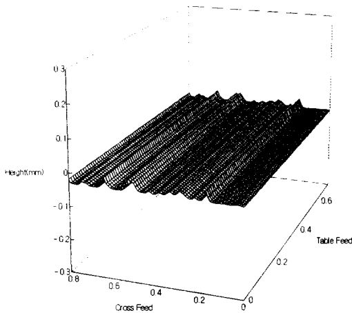
Fig. 6 Simulated surface roughness after 10 passes
