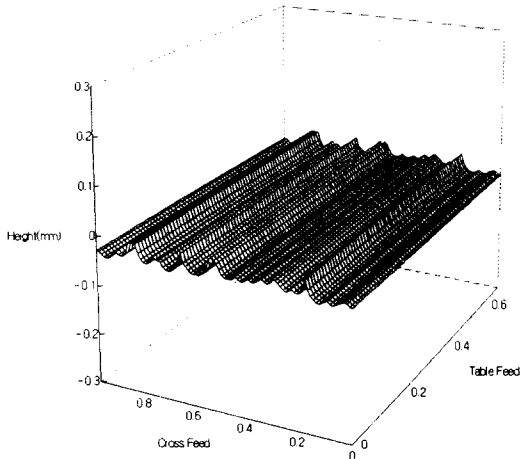
Fig. 5 Simulated surface roughness after dressing
