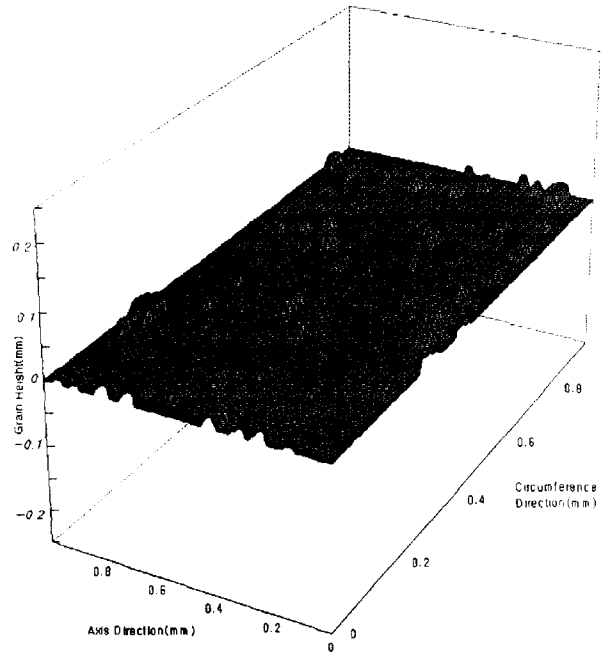
Fig. 4 Simulated grains on the grinding wheel after 10 passes
