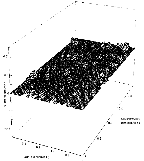
Fig. 3 Simulated grains on the grinding wheel after dressing
