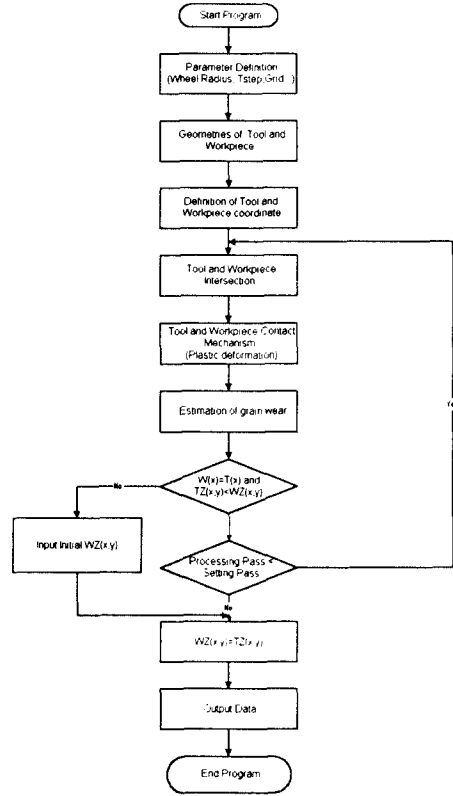
Fig. 1 Flowchart of the surface-shaping System
