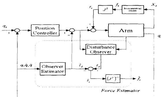
Fig.4 The block diagram of force estimator
