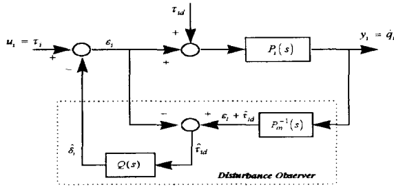
Fig.1. A structure of disturbance observer
