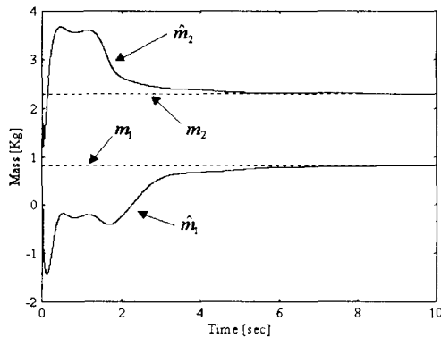
Fig. 6 The mass estimation of observer estimator
