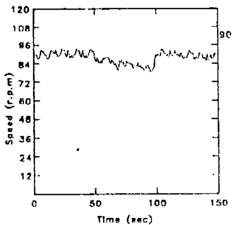
(a) PI Controller
