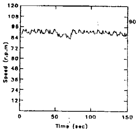
(b) Fuzzy Controller
