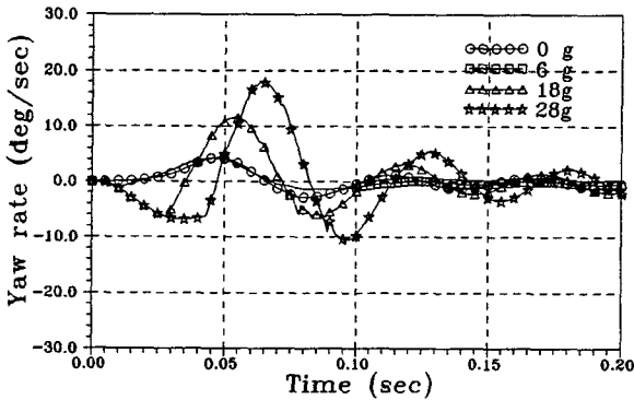
(b) Yaw rate of the launcher
