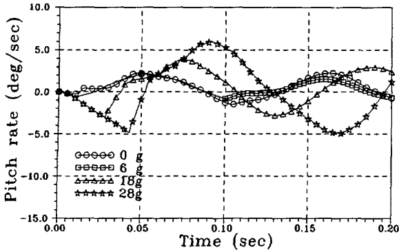
(a) Pitch rate of the launcher
