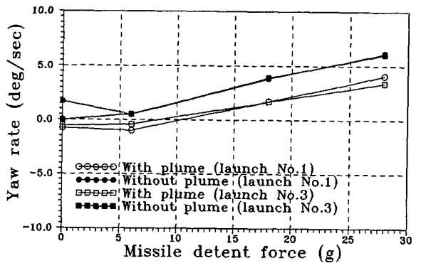
(b) Yaw rate of the missile
