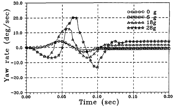
(a) Launch No. ①
