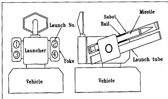
Fig. 1 Configuration of the Launcher system
