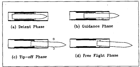
Fig. 2 Model of launching phase
