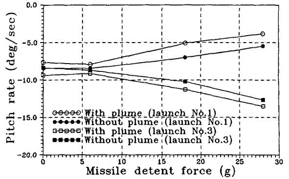
(a) Pitch rate of the missile
