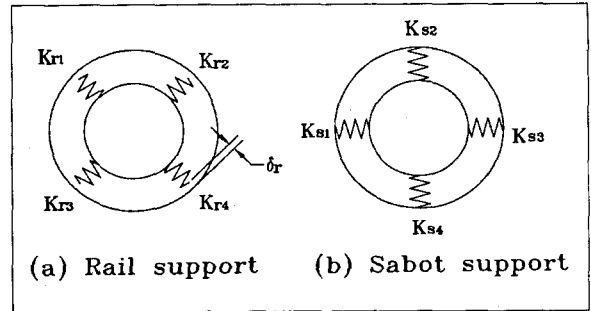
Fig. 3 Model of the missile support in the launch tube
