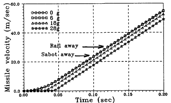
Fig. 4 Missile velocity as a function of detent force
