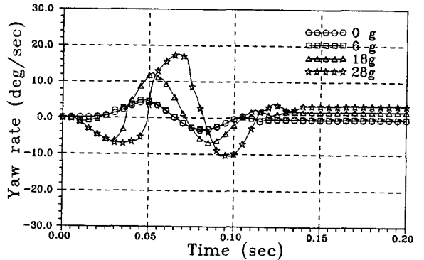
(b) Launch No. ③
