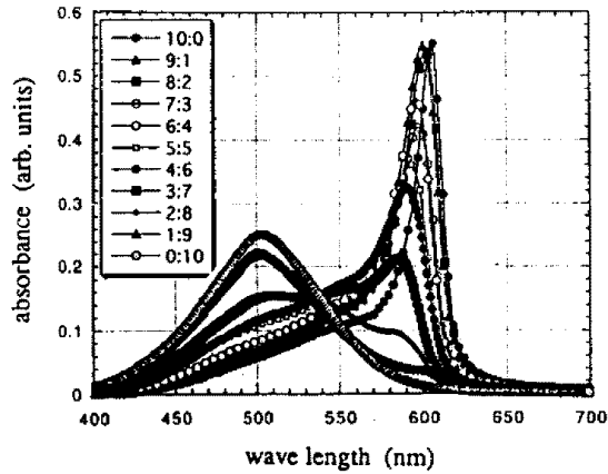
Fig. 5. Optical absorbance spectra of mixed LB film for concentration ratio.
