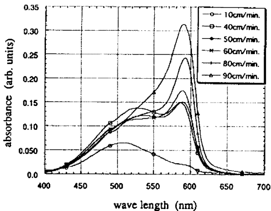
Fig. 6. Optical absorbance spectra of mixed LB film by compress speed of barrier.
