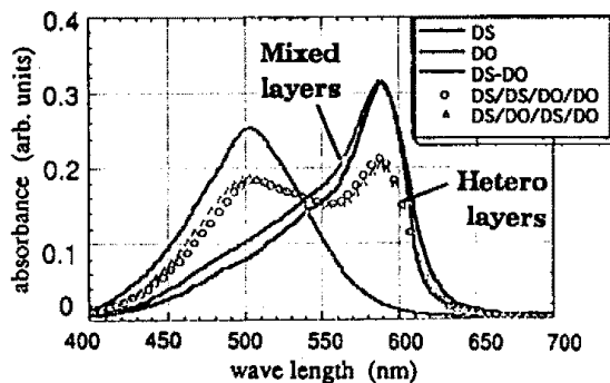
Fig. 4. Optical absorbance spectra of mixed & hetero LB film.
