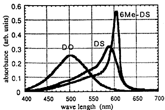
Fig. 2. Optical absorbance spectra of merocyanine
