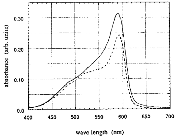
Fig. 7. Optical absorbance spectra of polarizer for mixed LB film.
