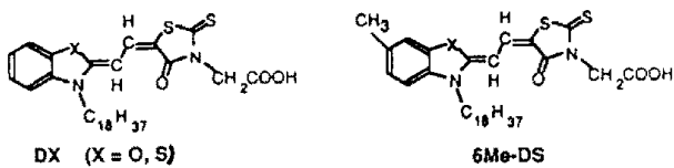
Fig. 1. Chemical structure of Molecular.
