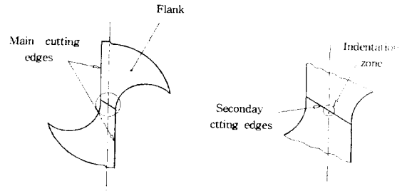
Fig.1 Shape of drill point
