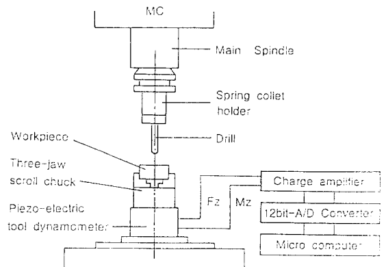
Fig.3 Schematic diagram of experiment
