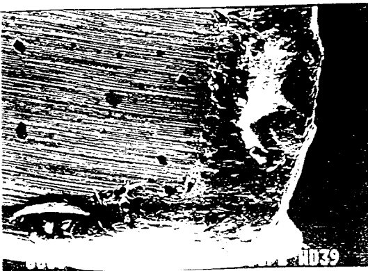
Fig.9 SEM Micrograph Of HSS-CO Tool
