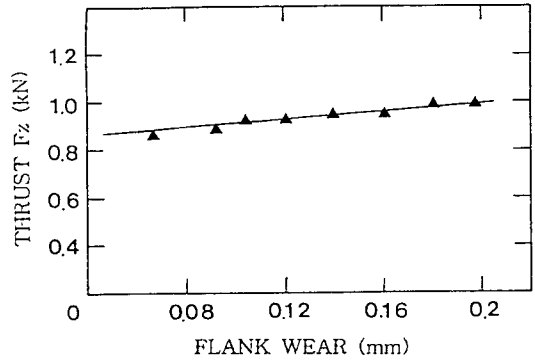
Fig.11 Flank wear versus thrust for HSS-CO ( V=7.8\text{m/min} , f=0.05\text{mm/rev} .)
