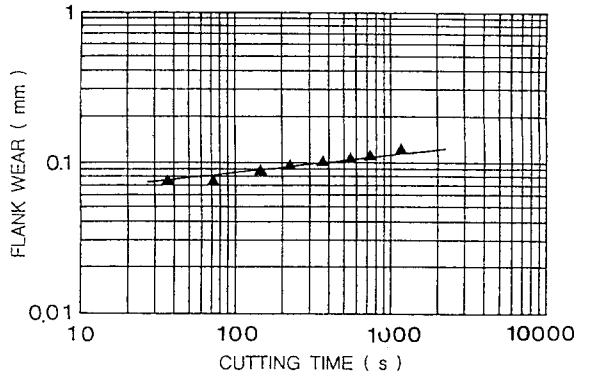
Fig.12 Flank wear versus cutting time for HSS+CO ( V=7.8\text{m/min} , f=0.05\text{mm/rev} .)
