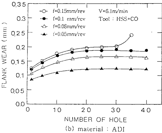
Fig.8 Comparison of tool wear in drilling ADI and GCD600 with cobalt contained HSS drill
