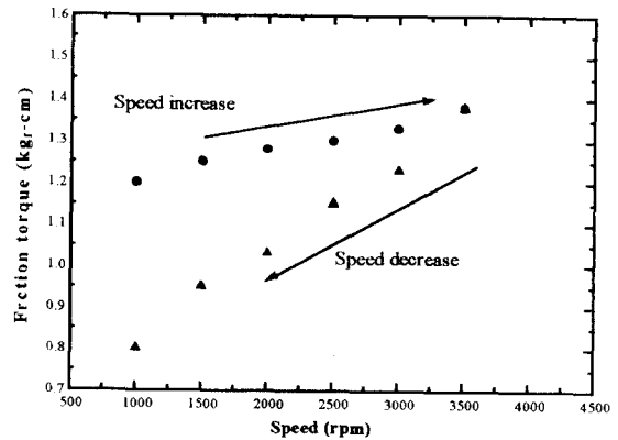
Fig. 3 Friction torque hysteresis for T_{oil} = 25^\circ\text{C} and P_{atm} .
