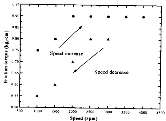
Fig. 5 Friction torque hysteresis for P_{vac} = 10^{-4} torr and T_{oil} = 25^\circ\text{C} .
