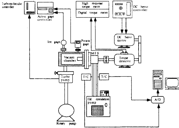
Fig. 2 Schematic of the testing equipment for measuring the friction torque of magnetic fluid seals.
