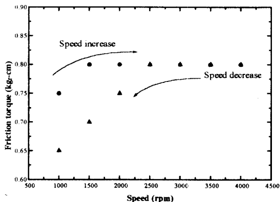
Fig. 7 Friction torque hysteresis for P_{vac} = 10^{-6} torr and T_{oil} = 25^\circ\text{C} .
