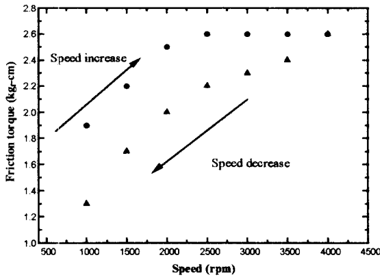
Fig. 13 Friction torque hysteresis for T_{oil} = 25^\circ\text{C} and P_{vac} = 10^{-6} torr.
