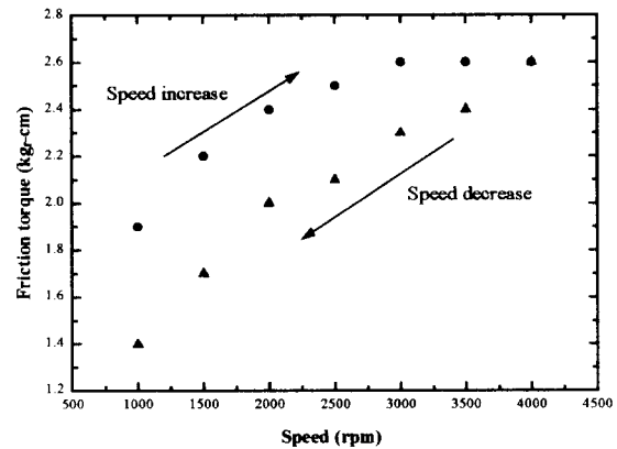
Fig. 11 Friction torque for T_{oil} = 25\text{ }^{\circ}\text{C} and P_{vac} = 10^{-4}\text{ torr} .
