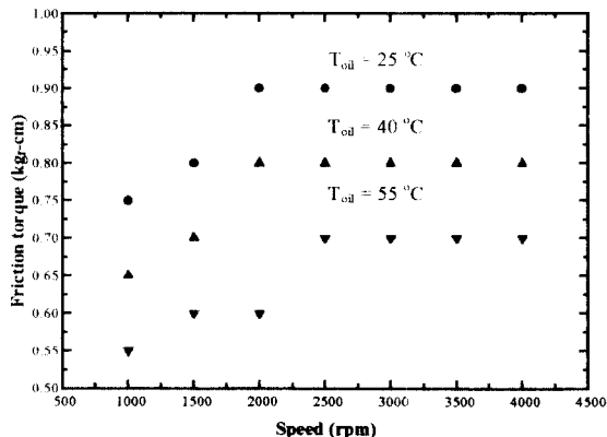
Fig. 6 Friction torque for various oil temperatures and P_{vac} = 10^{-4} torr.
