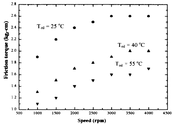
Fig. 14 Friction torque for various oil temperatures and P_{vac} = 10^{-6} torr.
