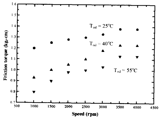
Fig. 4 Friction torque for various oil temperatures and P_{atm} .
