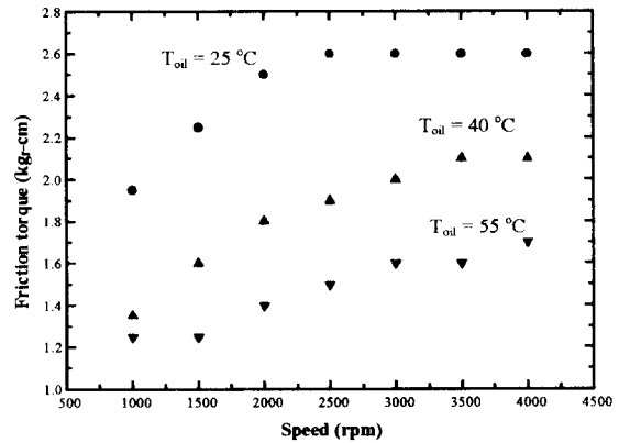
Fig. 10 Friction torque for various oil temperatures and P_{atm} .
