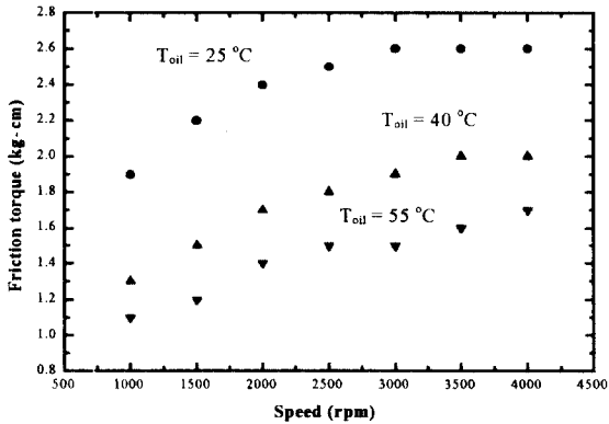
Fig. 12 Friction torque for various oil temperatures and P_{vac} = 10^{-4} torr.
