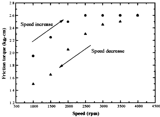
Fig. 9 Friction torque hysteresis for T_{oil} = 25\text{ }^{\circ}\text{C} and P_{atm} .
