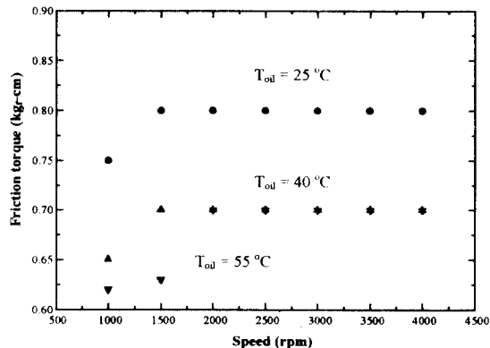
Fig. 8 Friction torque for various oil temperatures and P_{vac} = 10^{-6} torr.
