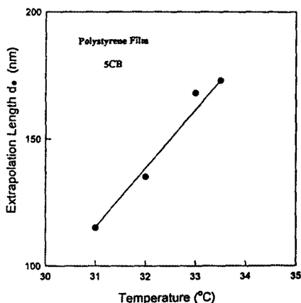
Fig. 3. Temperature dependence of extrapolation length in 5CB on rubbed polystyrene surface for strong rubbing (RS=406 mm). ( T_c=35.3^\circ\text{C} )
