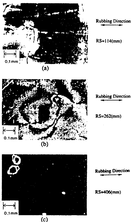
Fig. 2. Microphotographs of the textures for NLC, 5CB, on three kinds of the rubbed polystyrene surfaces. (a) RS = 114 mm; (b) RS = 262 mm; (c) RS = 406 mm.
