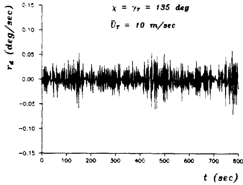
Fig. 12 Time history of disturbance due to wave and wind (ore carrier)
