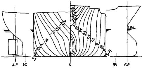
Fig. 3 Body plan and hull end profiles(ore carrier)
