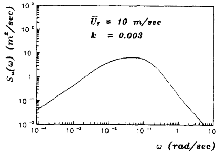
Fig. 9 Davenport wind spectrum
