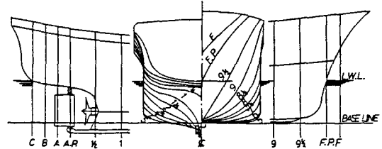
Fig. 4 Body plan and hull end profiles(fishing boat)
