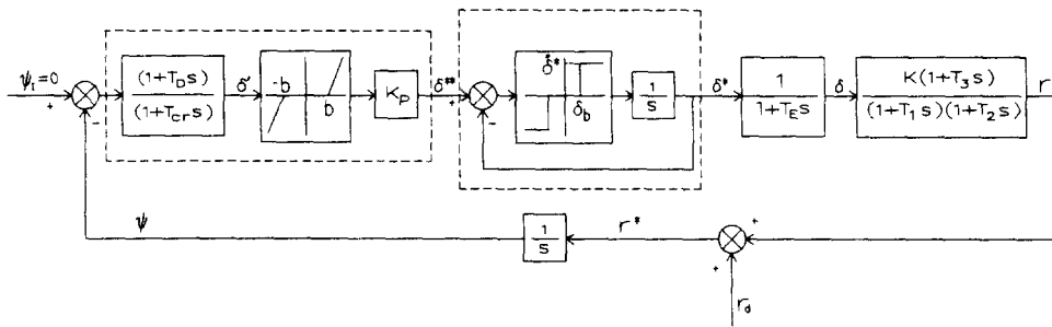
Fig. 2 Transfer functions of automatic steering system
