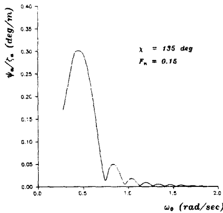
Fig. 6 Response amplitude operator of yaw(ore carrier)
