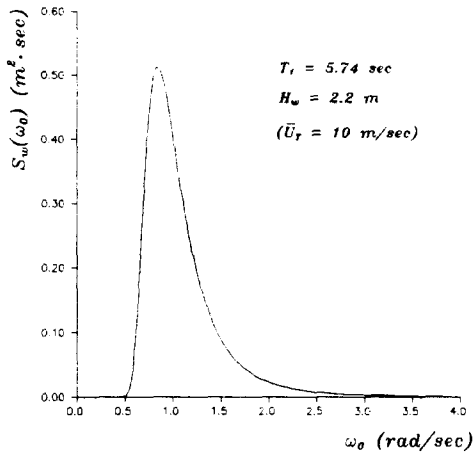
Fig. 8 ISSC wave spectrum
