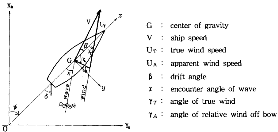
Fig. 5 Coordinate system and sign definition
