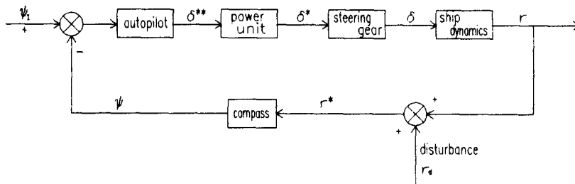
Fig. 1 Block diagram of automatic steering system
