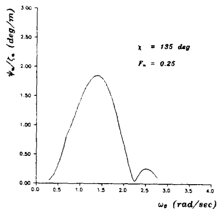
Fig. 7 Response amplitude operator of yaw(fishing boat)
