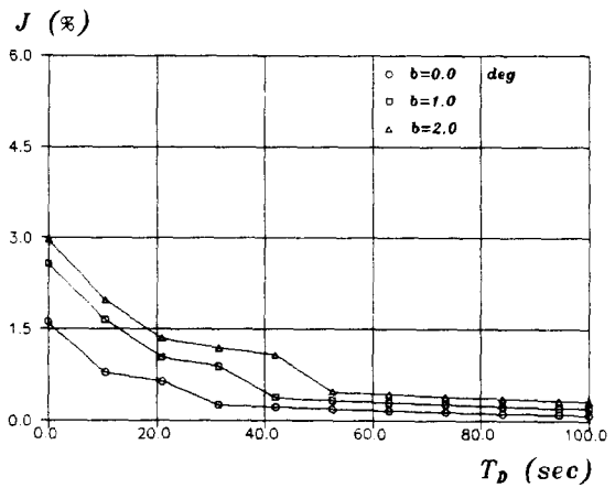
Fig. 19 The effect of weather adjuster on propulsive energy loss (ore carrier, T_{cr} = 10.5 \text{ sec} , K_P = 0.5 )
