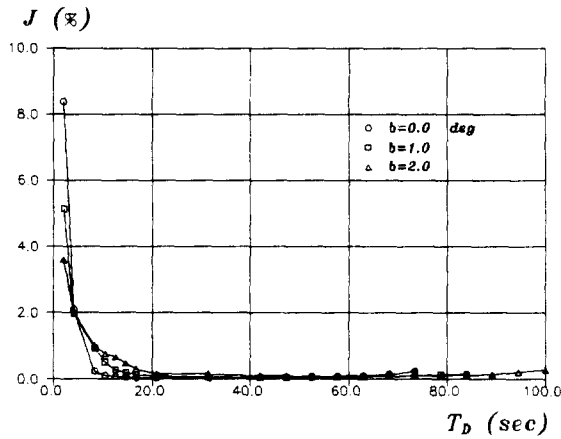
Fig. 18 The effect of weather adjuster on propulsive energy loss (fishing boat, T_{cr} = 10.5 \text{ sec} , K_P = 0.5 )
