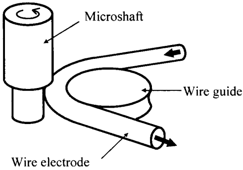
Fig.1 Principle of WEDG
