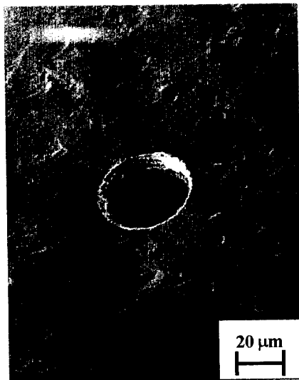
Fig.9 Machined microhole (Diameter 30\mu\text{m} , Depth 200\mu\text{m} , Brass)
