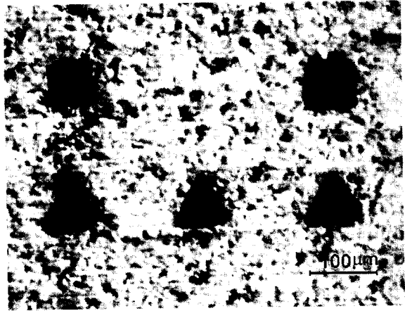
Fig.10 Machined micro polygon hole
