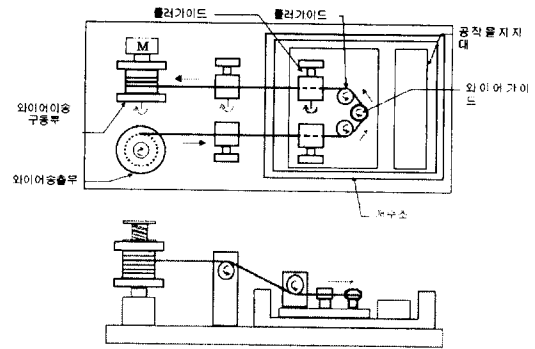
Fig. 5 Wire electrode driving device
