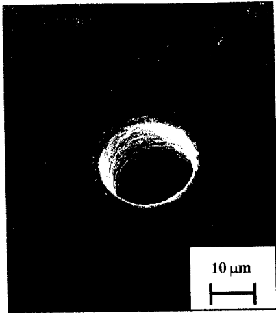
Fig.8 Machined microhole (Diameter 20\mu\text{m} , Depth 50\mu\text{m} , SUS304)
