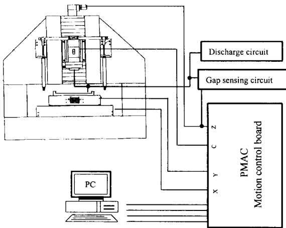
Fig.2 Schematic diagram of machining
