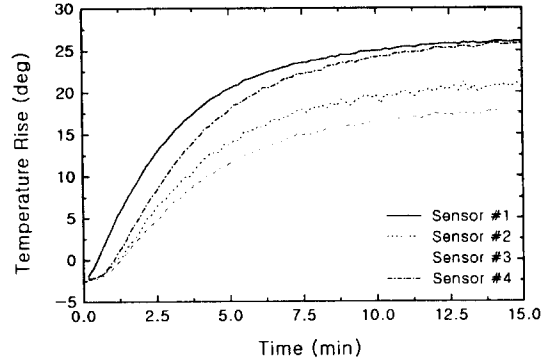
Fig.4 Temperature rise of spindle system (25,000rpm, 4 l/min/Brg)
