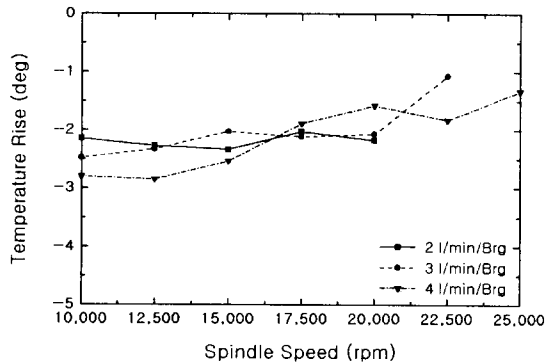
Fig.9 Temperature rise of oil tank
