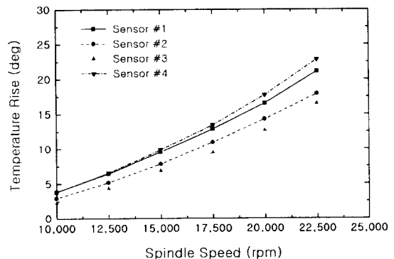
Fig.6 Temperature rise of spindle system (3 l/min/Brg)
