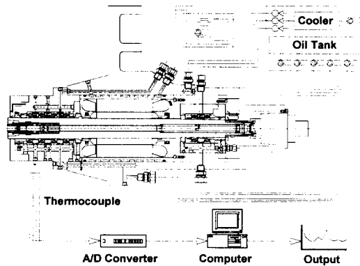
Fig.1 Schematic diagram for oil-jet lubrication testing
