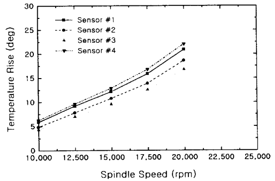
Fig.5 Temperature rise of spindle system (2 l/min/Brg)
