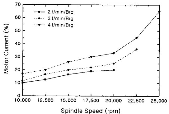
Fig.10 Motor current
