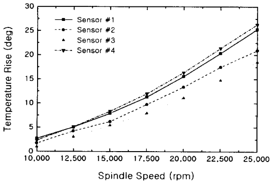
Fig.7 Temperature rise of spindle system (4 l/min/Brg)
