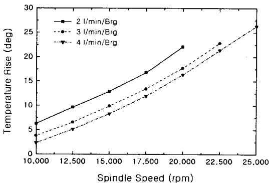
Fig.8 Temperature rise of spindle system (Sensor #1)
