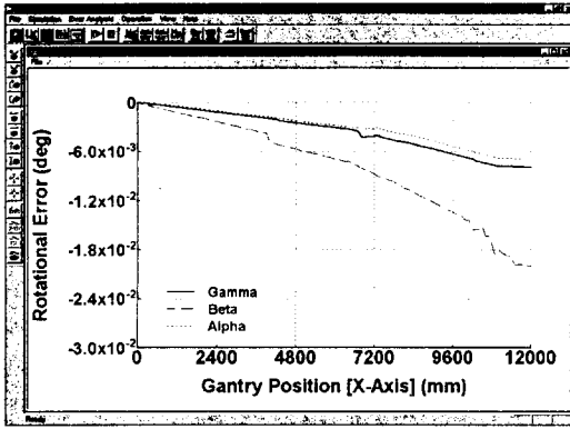
Fig.6 Rotational errors of gantry
