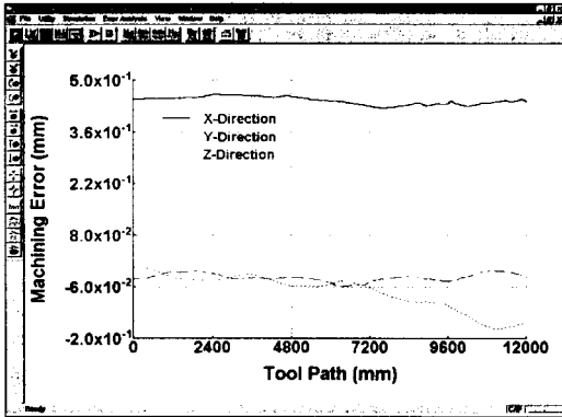
Fig.7 Machining error for linear interpolation
