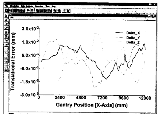
Fig.5 Translational errors of gantry
