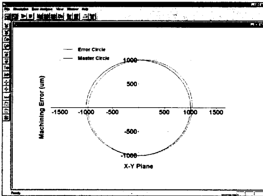
Fig.8 Machining error for circular interpolation
