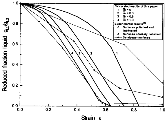
Fig. 3 Liquid fraction on strain for various friction condition at centerline
