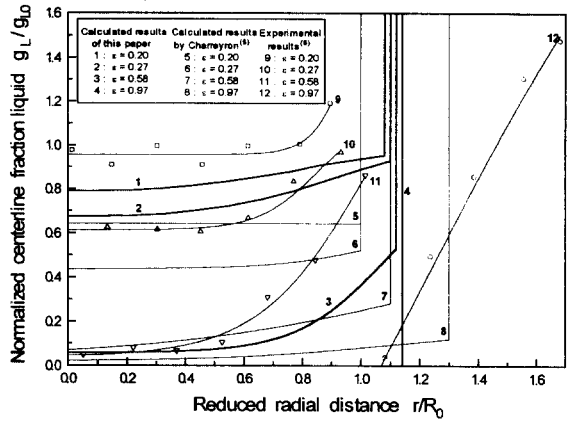
Fig. 2 Radial distribution of the liquid for Sn-15%Pb compressed at various strains ( \bar{m} = 1.0 )
