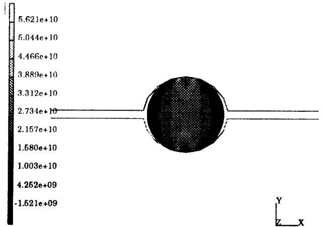
Fig. 10 Equivalent von Mises stress distribution of the multi-body contact mode in ball type slewing ring bearings.
