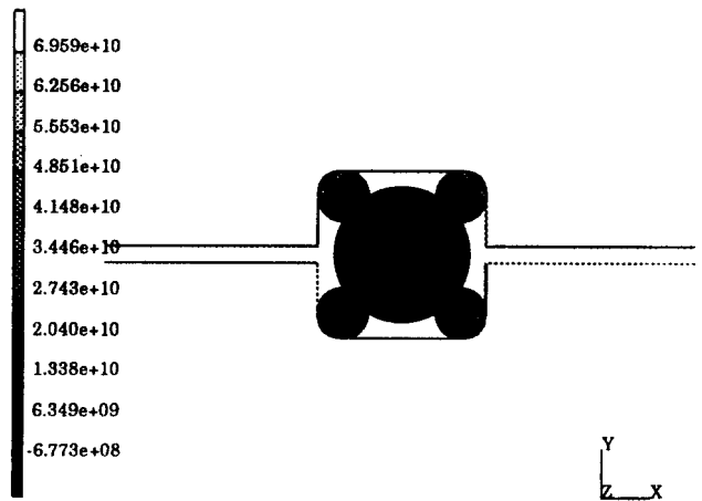
Fig. 11 Equivalent von Mises stress distribution of the multi-body contact mode in ball type wire race slewing ring bearings.
