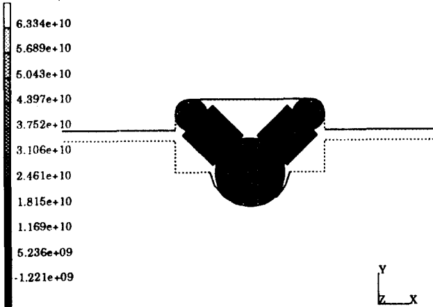
Fig. 12 Equivalent von Mises stress distribution of the multi-body contact mode in roller type wire race slewing ring bearings.
