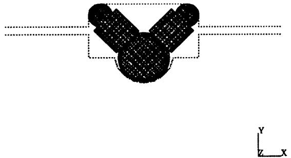
Fig. 7 Mesh generation for two rollers-triple wire race type of slewing ring bearings.
