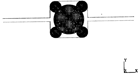
Fig. 6 Mesh generation for a ball-four wire race type of slewing ring bearings.
