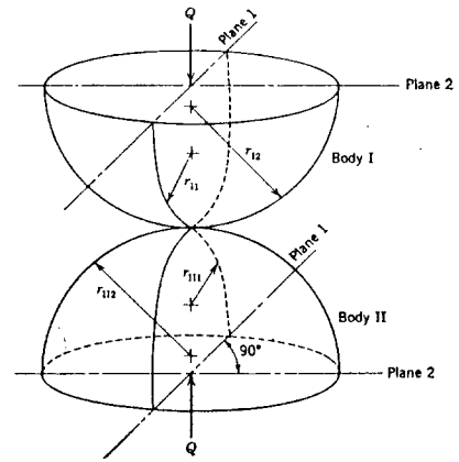
Fig. 1 Geometry of contact bodies.
