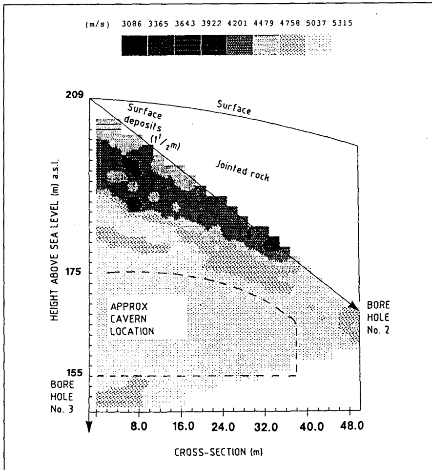
Fig.3 An example of cross-hole seismic tomography for extrapolating data between boreholes: Gjovik Olympic cavern.
