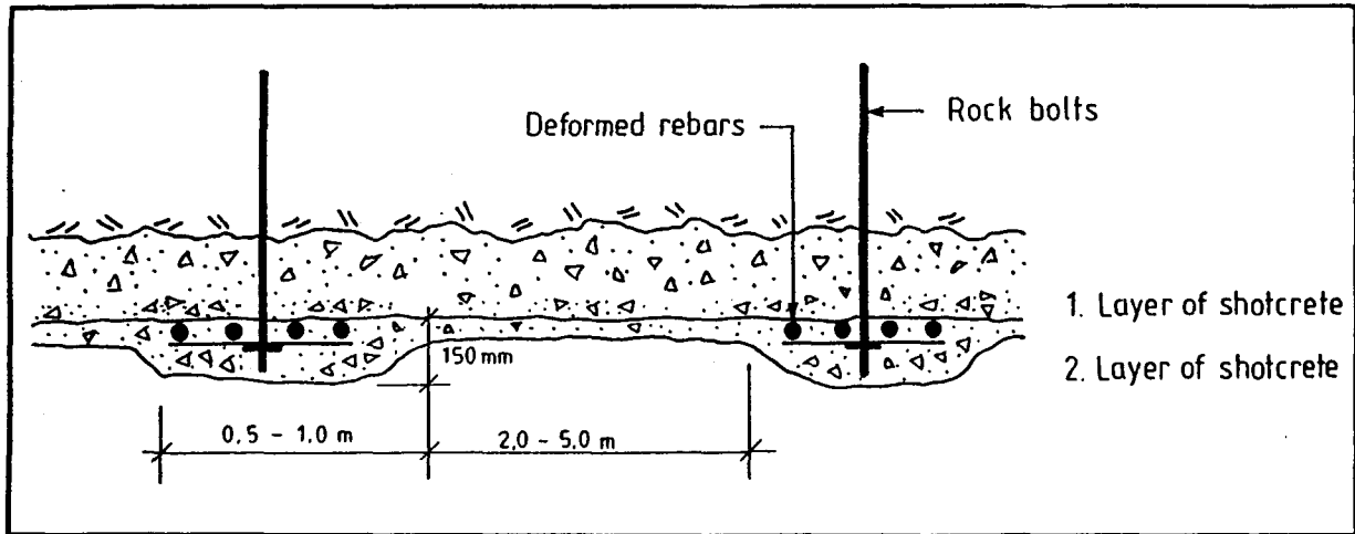
Fig.4 Support with ribs of reinforced shotcrete(RRS)
