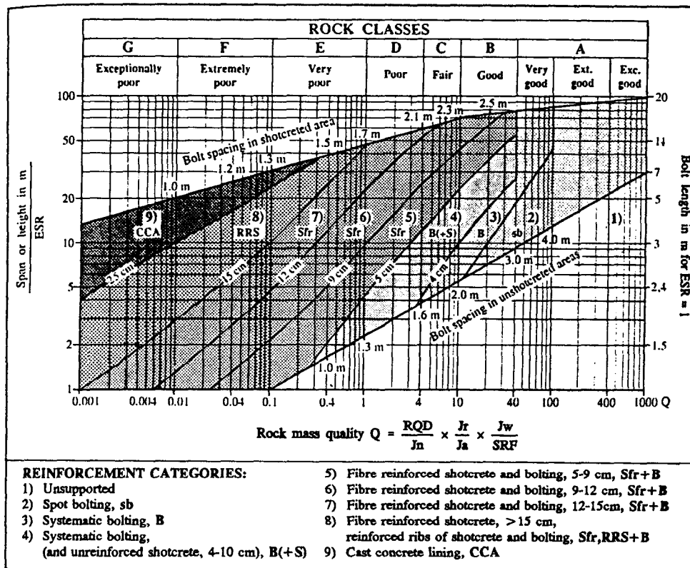
Fig.1 Rock mass classification-permanent support recommendation based on Q and NMT. (Note extensive use of S(fr) as permanent support.)
