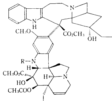
(1) vinblastine (R = CH 3 ) (2) vincristine (R = CHO)
