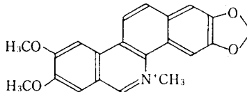
(10) nitidine chloride
