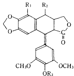
(11) podophyllotoxin (R 1 = H, R 2 = OH, R 3 = CH 3 )
