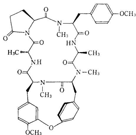
RA-IX
