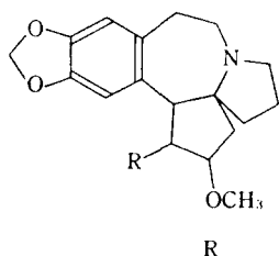
(6) -OH (7) \text{CH}_3-\underset{\text{CH}_3}{\overset{\text{OH}}{\text{C}}}-(\text{CH}_2)_2-\underset{\text{COO}}{\overset{\text{OH}}{\text{C}}}-\text{CH}_2-\overset{\text{O}}{\parallel}{\text{C}}-\text{OCH}_3
