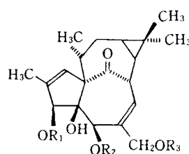
(14) ingenol-3-hexadecanoate (R 1 = CO(CH 2 ) 15 CH 3 , R 2 = R 3 = H)
