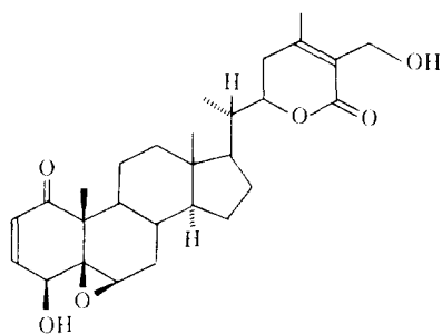
(20) withaferin A
