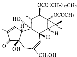
(13) 12-O-tetradecanoyl-phorbol-13-acetate (TPA)
