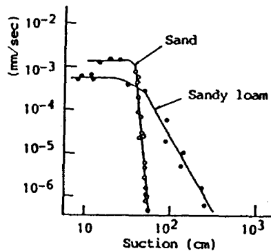
Fig.3.2 Permeability coefficient of unsaturation.
