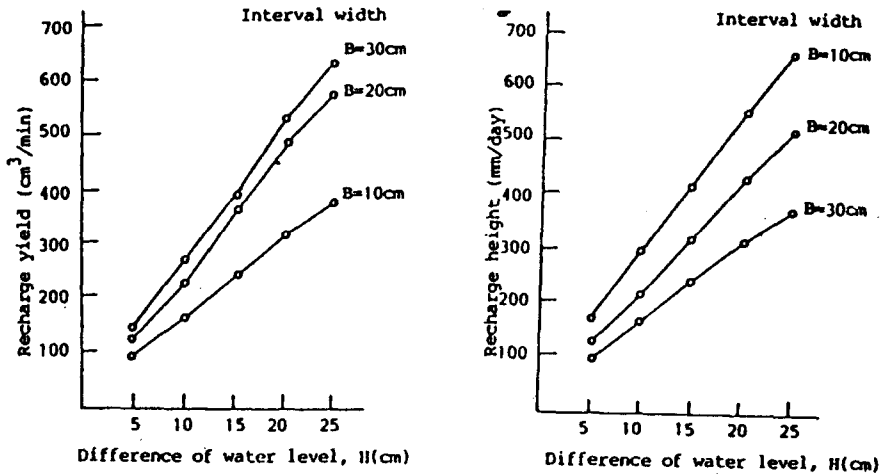
Fig.4.2 Experiment value for indoor experiment.
