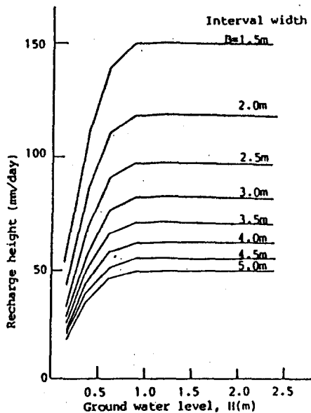
Fig. 4.6. The result of numerical analysis for field scale.
