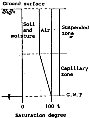
Fig. 2.1. The three phases distribution of soil
