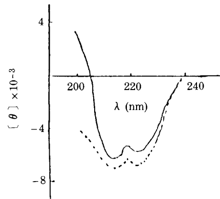
Fig. 2. CD spectra of Ginseng peptide solution at the different conditions. —, aqueous; ----, 1% SDS solution.
