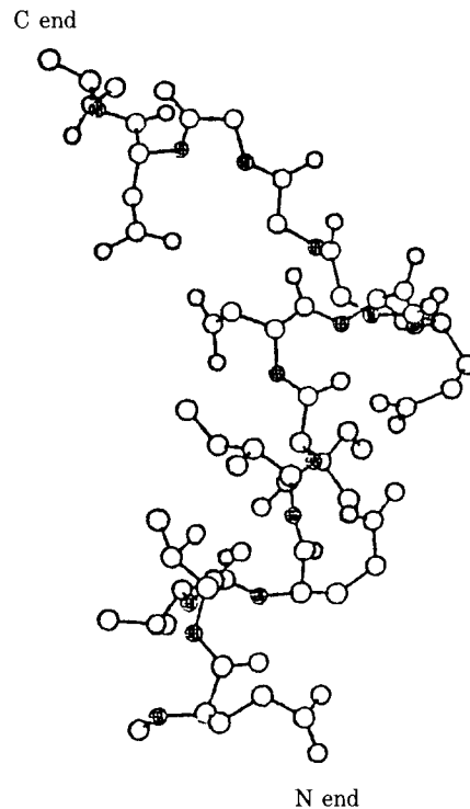
Fig. 3. Molecular model of Ginseng lpeptide ●-----N.
